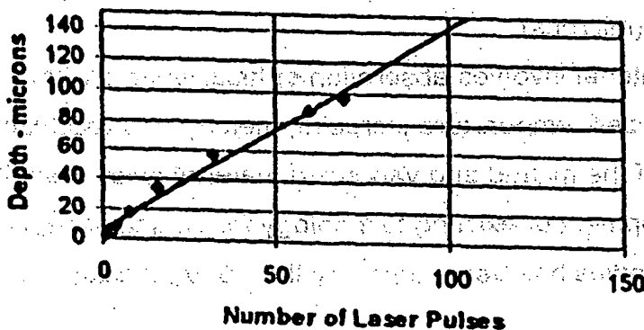
CUTTING DEPTH IN FORMING GAS AS A FUNCTION OF LASER PULSES
